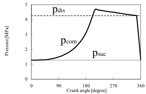
Figure4. Pressure of compression chamber
