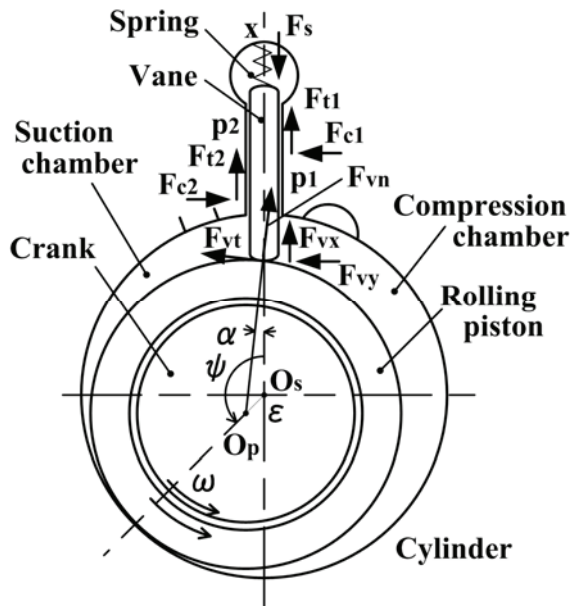
Figure1. Brief drawing of compression mechanism in rotary compressor
