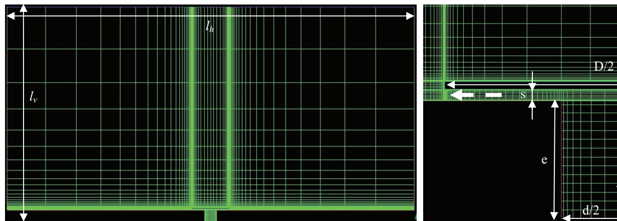
Figure 1. Mesh and computational domain. General view (left); zoom view (right).
