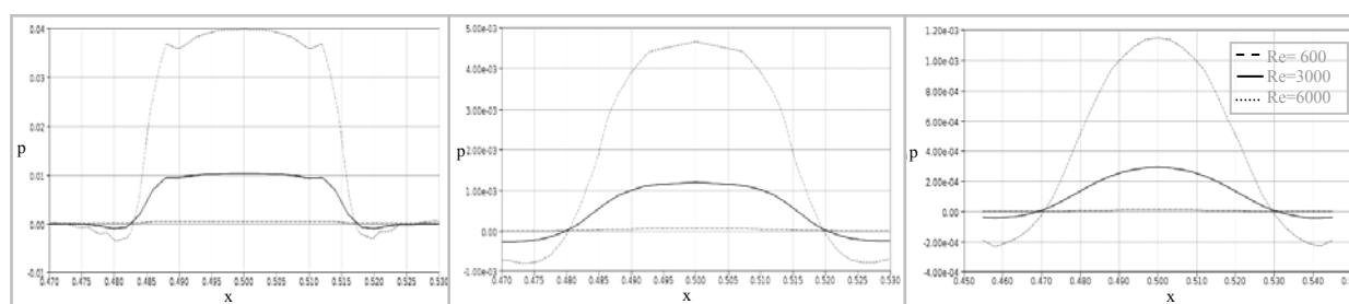
Figure 2. Comparative numerical analysis of Re influence for s/d ratios of 0.1, 0.4 and 0.9, respectively.
