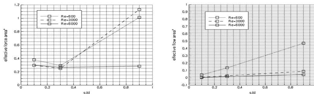
Figure 5. Numerical results globally evaluated as effective force and flow areas.
