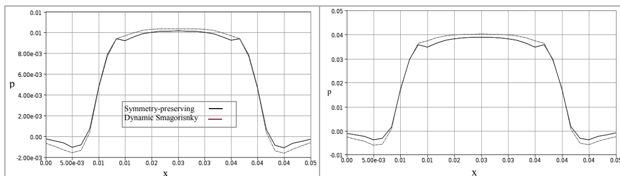
Figure 4. Comparative numerical analysis 3D periodic comparing symmetry-preserving vs. dynamic Smagorinsky turbulence modelling, for Re numbers of 3000 and 6000, respectively.
