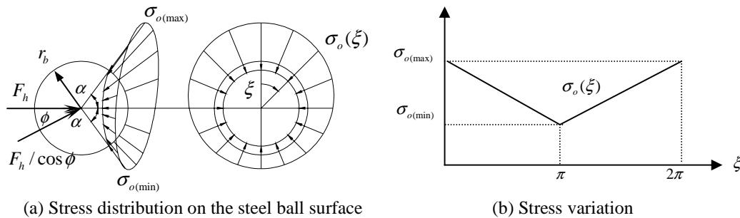
Figure 2.2 Stress distribution on the ball surface
