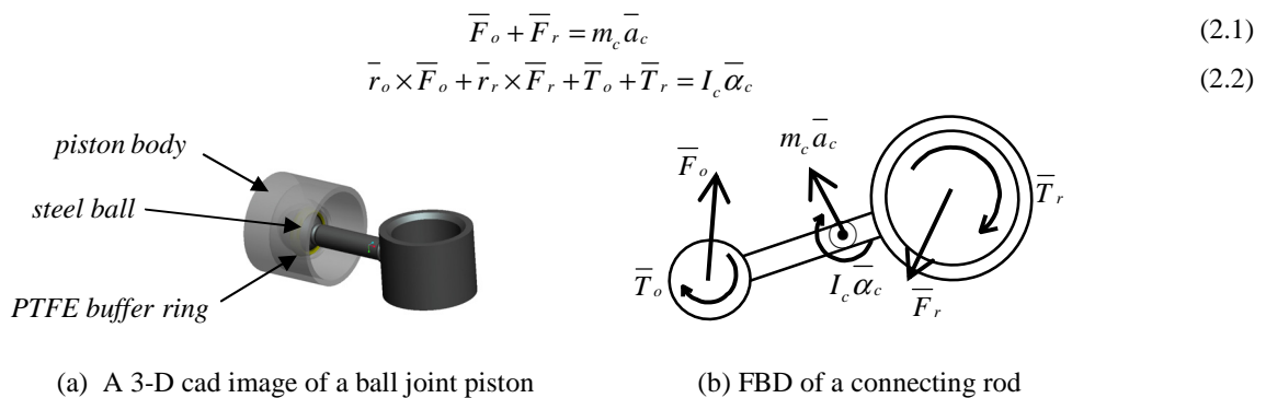
Figure 2.1 A ball joint type piston
