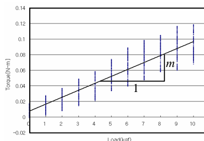
Figure 4.1 Relation between applied forces and friction torques
