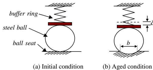
Figure 2.3 Ball joint configurations before and after the aging
