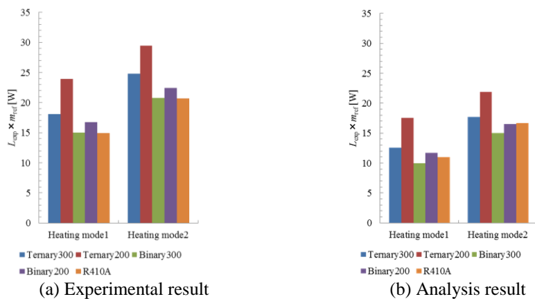
Figure 11: Irreversible loss through expansion valve
