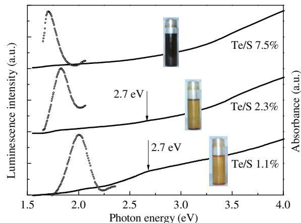
Figure 2. Room-temperature UV-visible absorption (solid lines) and photoluminescence (dotted lines) spectra of CdS:Te QDs with different Te/S molar ratios. Inset: photograph of three CdS:Te QDs in toluene in glass tubes.
