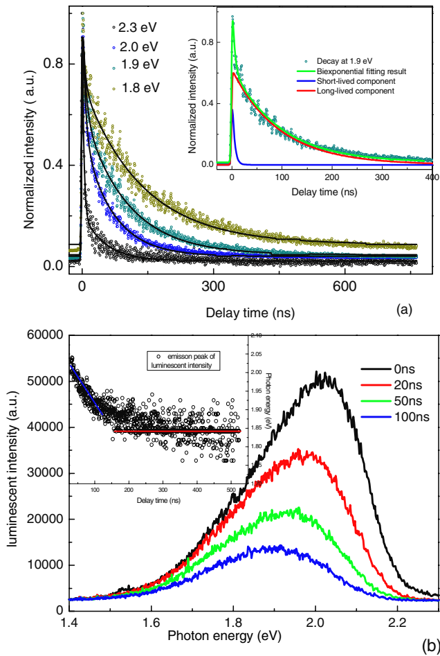
Figure 3. (a) PL decay curves of CdS:Te:1.1% QDs for photon energies of 2.3, 2.0, 1.9 and 1.8 eV, respectively. The solid lines are exponential fitting curves of experimental data. Inset: corresponding experimental result, its biexponential fitting, long-lived component, and short-lived component. (b) Temporal evolution of PL spectra from 0 to 100 ns from top to bottom. Inset: the spectra are shifted vertically and the times are indicated in the graph.
