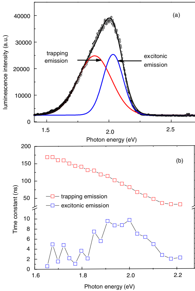
Figure 5. (a) The luminescence spectrum of CdS:Te QDs with a Te/S molar ratio of 1.1%. It can be decomposed into a higher-energy component (blue) due to excitonic emission and a lower-energy component due to trapping state emission (red). (b) Lifetime of the excitonic and trapping state emissions as a function of photon energy.
