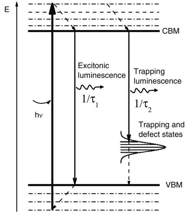
Figure 4. Energy level diagram of CdS:Te QDs, where trapping and defect states are shown. CBM, conduction band minimum; VBM, valence band maximum.
