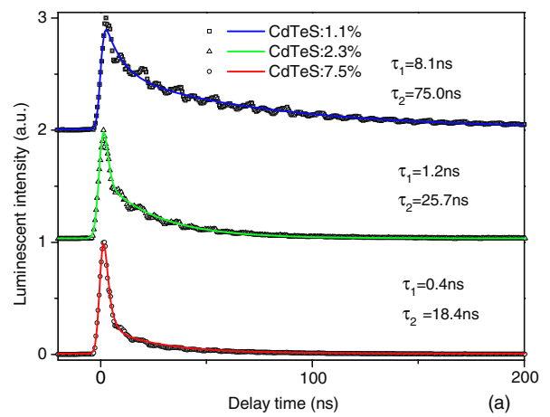
Figure 6. Normalized luminescence decay curves of three CdS:Te QD samples at 400 nm laser excitation. The decays of three different CdS:Te QDs are integrated about 30 nm near the emission peak.
