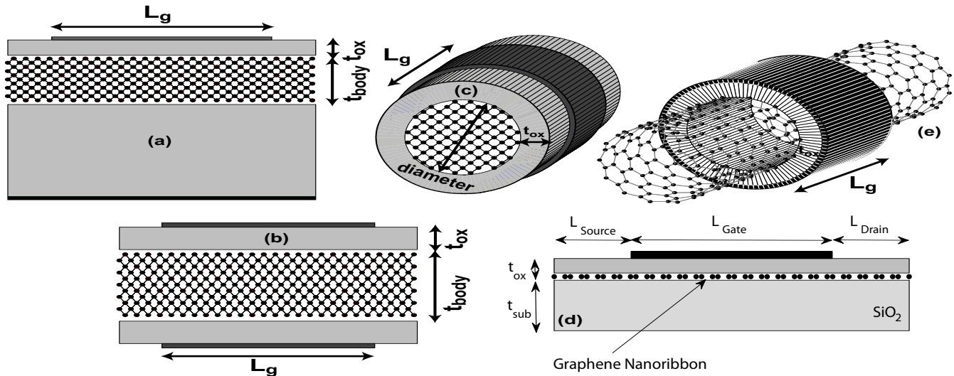
Fig. 1. Schematic view of the different p-i-n tunneling FETs considered in this work. (a) Single-Gate Ultra-Thin-Body (SG UTB), (b) Double-Gate Ultra-Thin-Body (DG UTB), (c) Gate-All-Around Nanowire (GAA NW), (d) Single-Gate Graphene Nanoribbon (SG GNR), and (e) Gate-All-Around Carbon Nanotube (GAA CNT). The UTB and NW are either made of pure InSb or of a relaxed GaSb-InAs heterostructure. In this case, the p -doped region is made of GaSb, the intrinsic channel and the n -doped side of InAs. The body thickness, the diameter, and the ribbon width of all the structures measure 5nm, except the CNT that has a diameter of 3.4nm ( \Rightarrow same band gap as GNR). All the devices are characterized by an EOT of 0.5nm (2nm thick dielectric with \epsilon_R=16 ).
