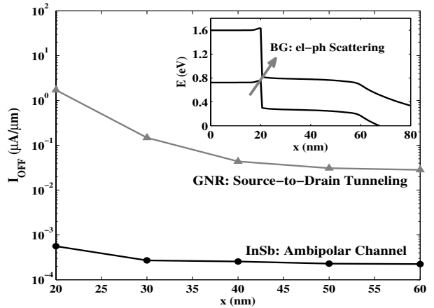
Fig. 11. OFF-current of the 5nm thick SG InSb UTB (black line with circles) and of the 5nm thick SG graphene NR (gray line with triangles) as a function of the channel length. The inset shows that the OFF-current of the GaSb-InAs broken gap heterostructure might be dominated by electron-phonon scattering and cannot be correctly modeled in the ballistic approximation.
