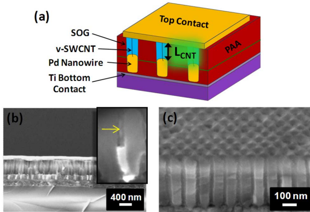
Fig. 2. (a) Schematic cross section of a two-terminal, multinanotube v-SWCNT device. (b) Cross-sectional SEM showing the vertical nanopores and Pd nanowire bottom contacts with a Pd/Ti/Au top contact. Inset shows a v-SWCNT supported in SOG with an arrow indicating the v-SWCNT location. (c) Tilted cross-sectional SEM showing the ordered nanopores prior to top contact metallization.
