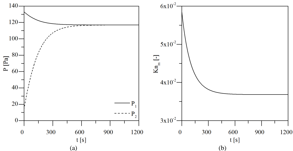
Figure 2: Data from a single experiment with R600a in a copper microtube: (a) variation of pressure in the reservoirs and (b) variation of Kn_m .
