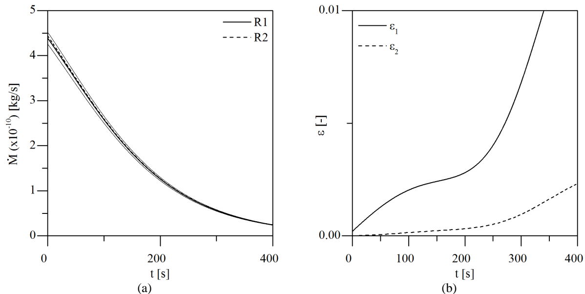
Figure 3: Data extracted from a single experiment with R600a in a copper microtube: (a) variation of the mass flow rates through the microtube and (b) variation of \epsilon .
