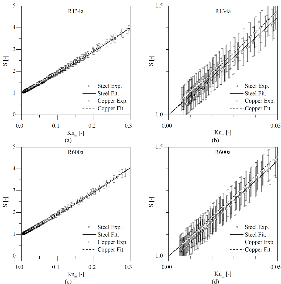
Figure 4: Non-dimensional mass flow rate as a function of Kn_m : (a)-(b) R134a and (c)-(d) R600a.
