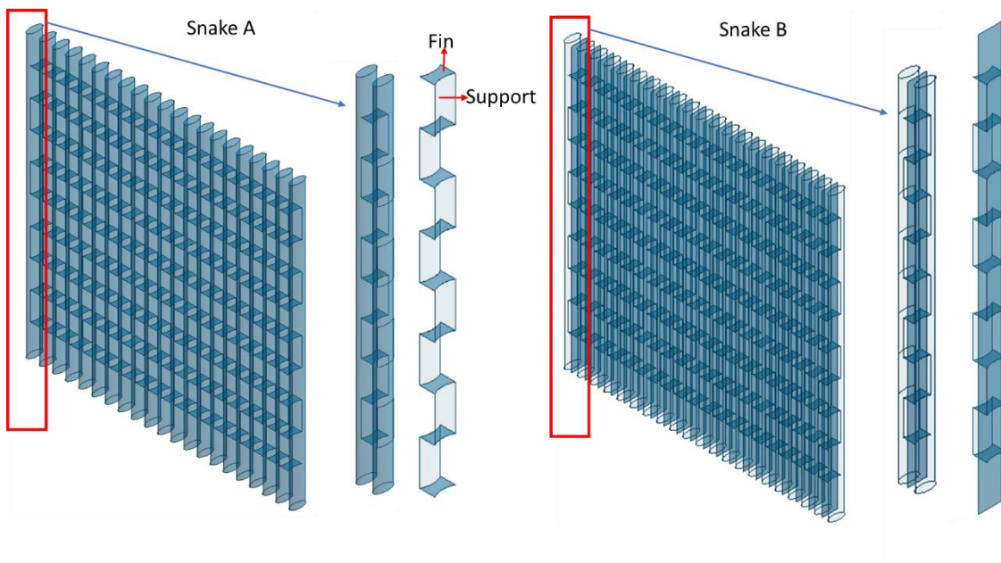
Figure 3: Two types of fins added to the tubes, Snake A and Snake B.
