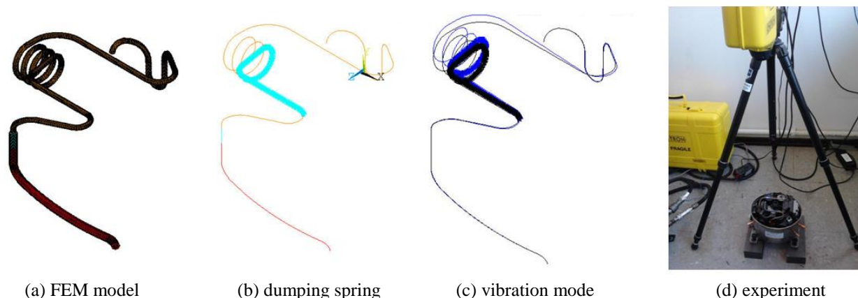
Figure 9: FEM analysis and validation
