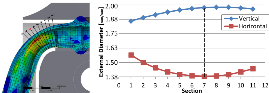
Figure 15: Discharge connector roundness deviation in first curvature
