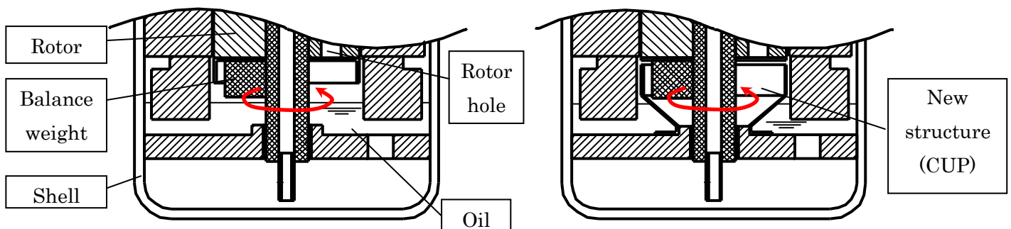
Fig. 2.1. Conventional structure
