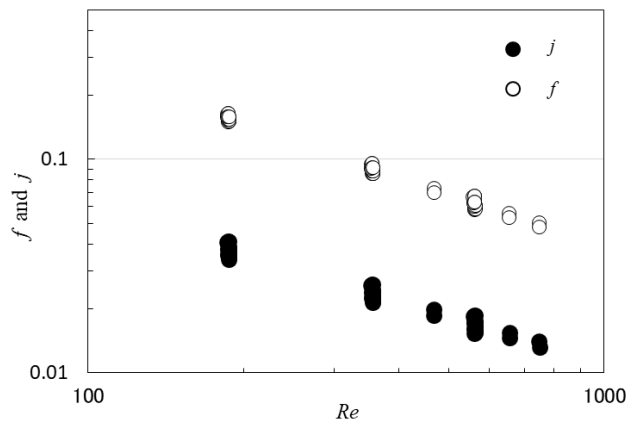
Figure 5: Dimensionless arrangements for the plane fins
