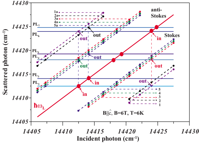
FIG. 5. (Color online) Scattered photon energies \hbar\omega_S of Raman EPR lines as a function of the incident photon energy \hbar\omega_L . As a convenient reference line for the Stokes and the anti-Stokes Raman shifts, \hbar\omega_L is also plotted along the diagonal of the figure, with all the \hbar\omega_S lines, thus, being parallel to the diagonal \hbar\omega_L line. The Raman transitions corresponding to each \hbar\omega_S line (1a–5a and 1–5) are given in the text. Full circles on the \hbar\omega_S lines denote the observed Raman shifts for B=6 T. The photoluminescence lines PL_2 – PL_7 , being independent of \hbar\omega_L , appear in the figure as horizontal lines parallel to the abscissa.
