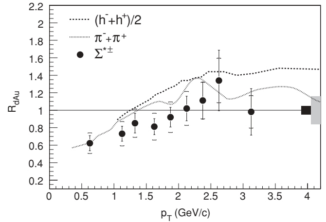
FIG. 37. Same as Fig. 35, but for \Sigma^* R_{dAu} .
