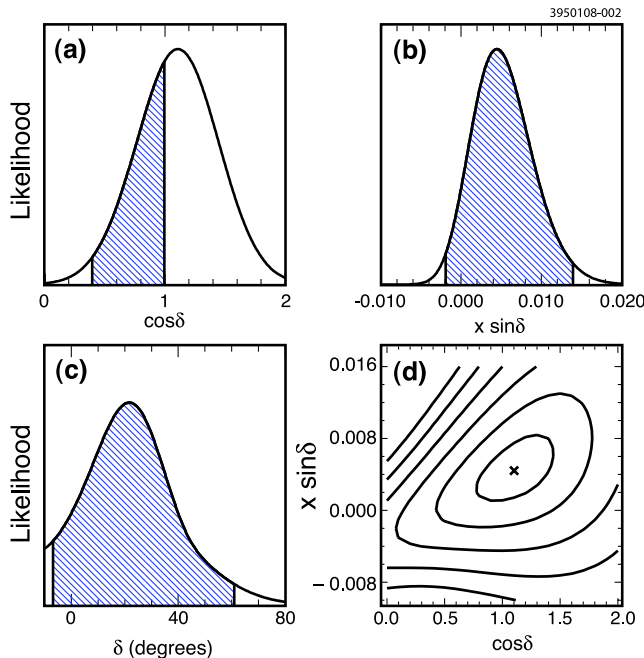
FIG. 2 (color online). Extended fit likelihood including both statistical and systematic uncertainties for \cos\delta (a), x\sin\delta (b), \delta (c), and simultaneous likelihood for \cos\delta and x\sin\delta (d) shown as contours in increments of 1\sigma , where \sigma = \sqrt{\Delta\chi^2} . The hatched regions contain 95% of the area in the physical regions. For \delta , the fit fails to converge beyond the limits of the plot.
