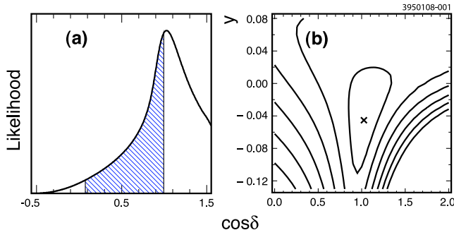
FIG. 1 (color online). Standard fit likelihood including both statistical and systematic uncertainties for \cos\delta (a), and simultaneous likelihood for \cos\delta and y (b) shown as contours in increments of 1\sigma , where \sigma = \sqrt{\Delta\chi^2} . The hatched region contains 95% of the area in the physical region.
