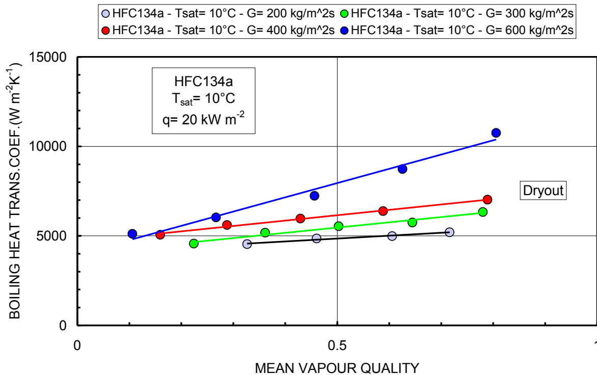
Figure 3b: Average heat transfer coefficient on refrigerant side vs. mean vapour quality and refrigerant mass flux at 10^\circ\text{C} of saturation temperature and 20 \text{ kW m}^{-2} of heat flux for HFC134a
