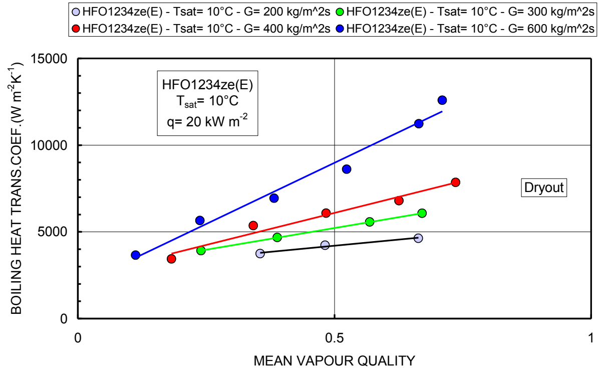
Figure 3a: Average heat transfer coefficient on refrigerant side vs. mean vapour quality and refrigerant mass flux at 10^\circ\text{C} of saturation temperature and 20 \text{ kW m}^{-2} of heat flux for HFO1234ze(E)
