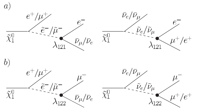
FIG. 1. Lowest order Feynman diagrams for \mathcal{R}_p SUSY decay of the LSP via virtual sleptons governed by (a) the \lambda_{121} coupling and (b) the \lambda_{122} coupling.
