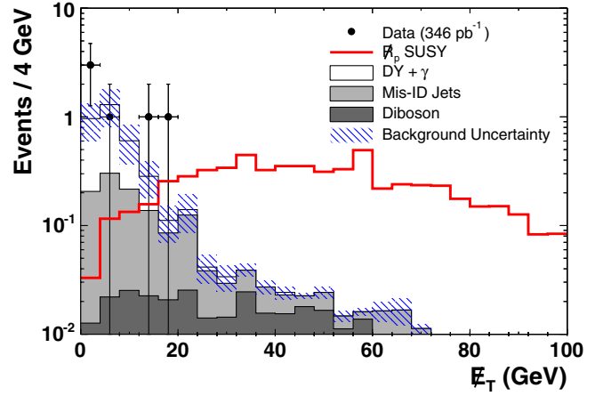
FIG. 2 (color online). \cancel{E}_T for events in the tripleton signal samples. For comparison, an \cancel{E}_p SUSY sample is shown with M(\tilde{\chi}_1^0) = 99 \text{ GeV}/c^2 .
