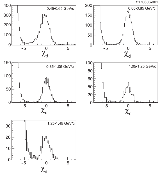
FIG. 2. Deuteron \chi_d distributions ( dE/dx normalized deviation) in different deuteron momentum bins.
