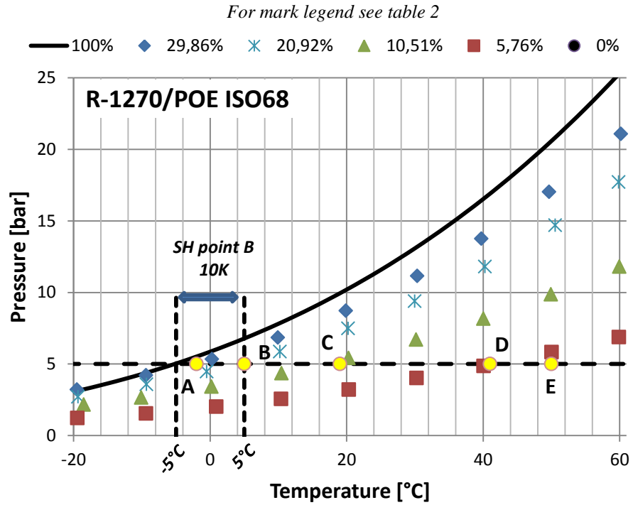
Figure 3: Pressure-temperature-concentration diagram
