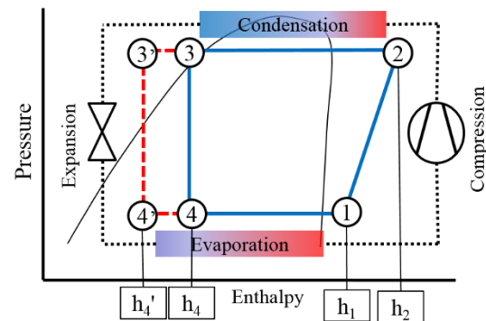
(b) p-h Diagram
