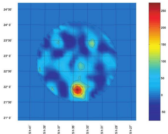
FIG. 2.—Gaussian-smoothed ( \sigma = 7.6' ) declination vs. right ascension map of the excess counts from the Crab Nebula observed with the 0.8^\circ offset toward north from the telescope optical axis for a total of 3.2 hr. The color bar represents the excess counts, and the coordinates are referenced to the epoch J2000.0.
