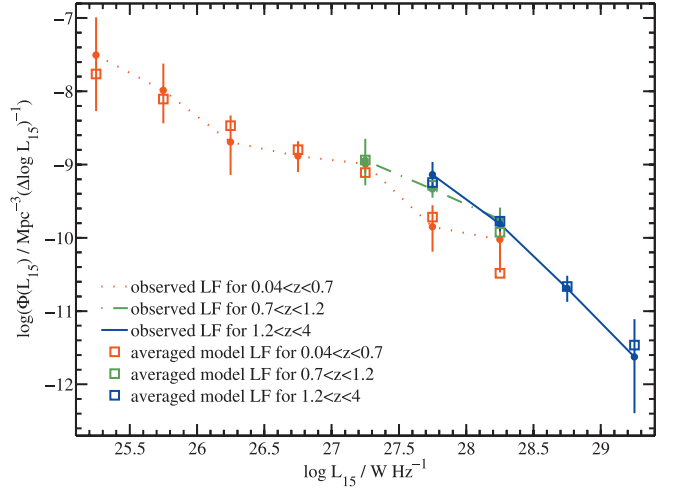
FIG. 4.— Observed binned RLF of the MOJAVE known FR II sample ( filled circles and lines ) and the binned model RLF ( open squares ) for three redshift intervals: 0.04 < z < 0.7 ( red, dotted line ), 0.7 < z < 1.2 ( green, dot-dashed line ), and 1.2 < z < 4 ( blue, solid line ). The luminosity bin width is \Delta \log L = 0.5 .
