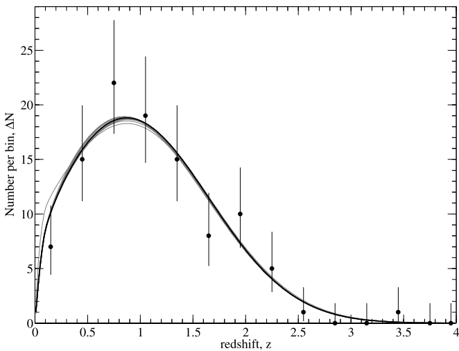
FIG. 3.— Plot of model redshift distributions for each redshift randomization ( thin light gray lines ), best-fit model distribution ( thick black line ), and the observed redshift distribution of the MOJAVE known FR II sample ( filled circles with error bars corresponding to 1\sigma confidence level ).
