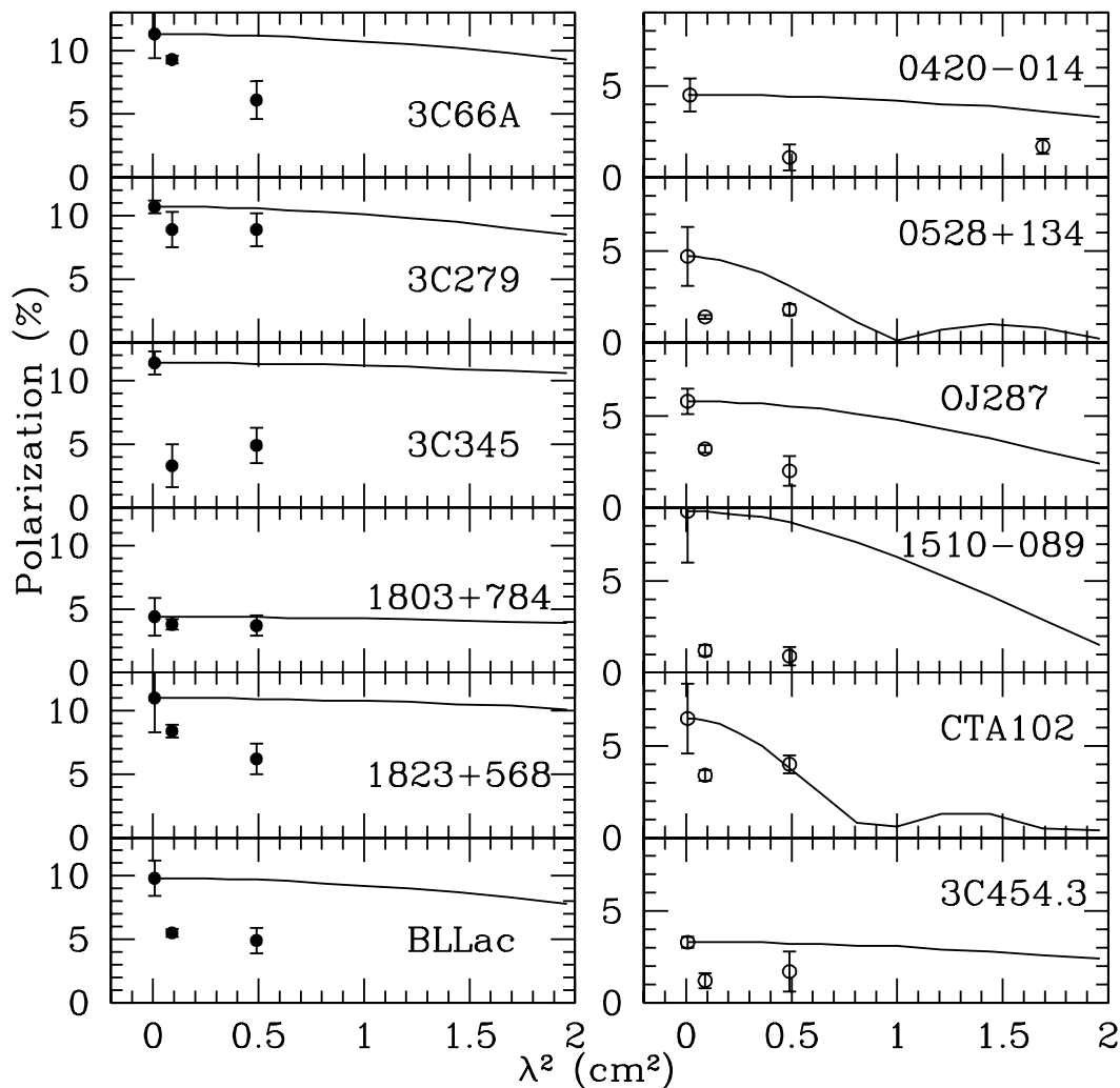
FIG. 14.—Dependence of degree of polarization on wavelength in the IVP (left) and HVP (right) sources. Solid lines represent the expected Faraday depolarization according to eq. (4) and RM derived in § 5.1. In general, the fit is poor, so that in most of our sources Faraday depolarization is unable to explain the frequency dependence of the polarization.
