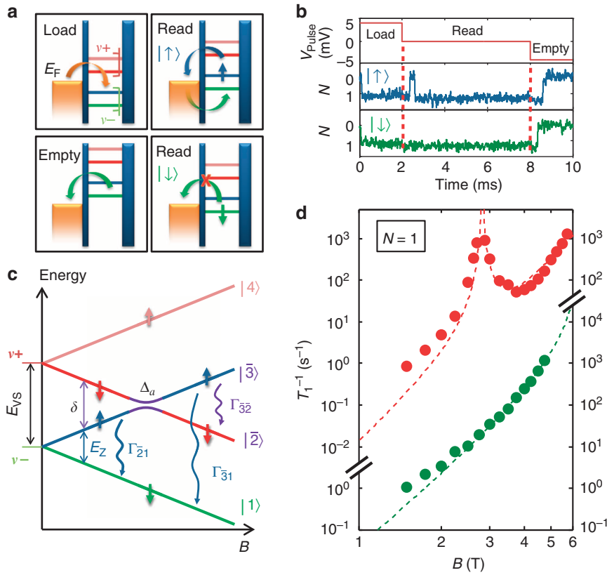
Figure 2 | Spin read-out and relaxation rates for single-electron occupancy. (a) Schematic diagram showing the effect of the three-level pulse sequence on the electrochemical potential of the dot. Energy levels in the QD are Zeeman split according to spin polarization and valley degeneracy is lifted. For clarity, only lower valley states are shown to be loaded/unloaded. (b) Pulsing sequence (top) for the single-shot spin read-out and normalised SET signal for spin-up (middle) and spin-down (bottom). (c) Energy diagram of the one-electron spin-valley states as a function of B field. Maximum mixing of spin and valley degrees of freedom occurs at the anticrossing point where Zeeman and valley splittings coincide. Relevant relaxation processes are sketched. (d) Relaxation rates as a function of magnetic field for different valley splittings. Data points for E_{VS} = 0.75 meV, E_{VS} = 0.33 meV are shown as green and red circles, respectively. Dashed lines are the calculated relaxation rates fitted with r = 1.7 nm (green), r = 1.1 nm (red).
