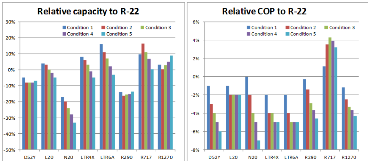
Figure 5: R-22/R-407C replacement candidates' relative performance to the baseline
