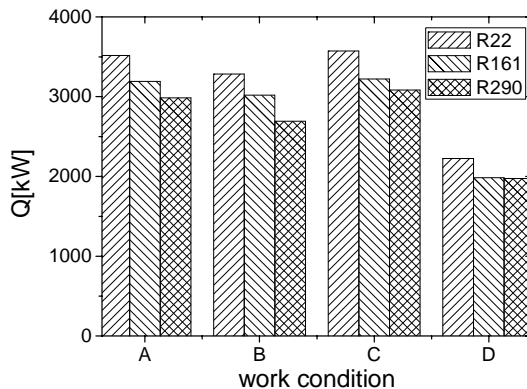
Fig 4: Cooling or heating capacity
