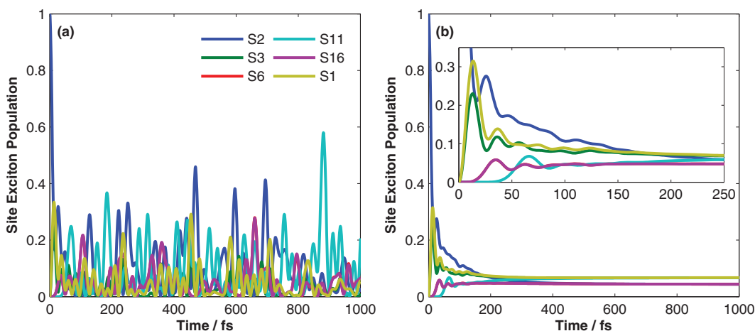
FIG. 3. The exciton population dynamics of B850 bacteriochlorophylls (BChls) with site 2 (S2) initially excited. (a) The population evolution of S1, S2, S3, S6, S11, and S16 without dissipation (the system is isolated and uncoupled to bath). (b) The population dynamics of the same sites while the system is coupled to bath at room temperature T = 300 K. The coherent energy transfer lasts about 150 fs and the whole system is equilibrated after 400 fs. The inset is a magnification of the first 250 fs-dynamics.
