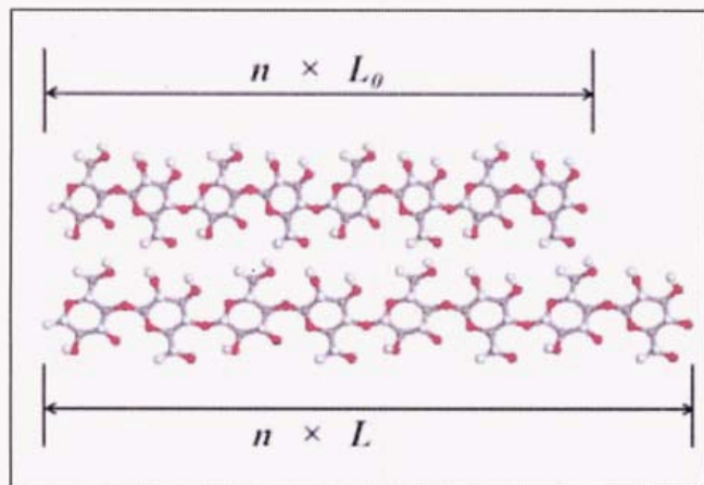
2. Snapshots of a model cellulose chain at its equilibrium and strained lengths where n is the number of repeat units. Atoms represented as grey (carbon), red (oxygen), and white (hydrogen) spheres.
