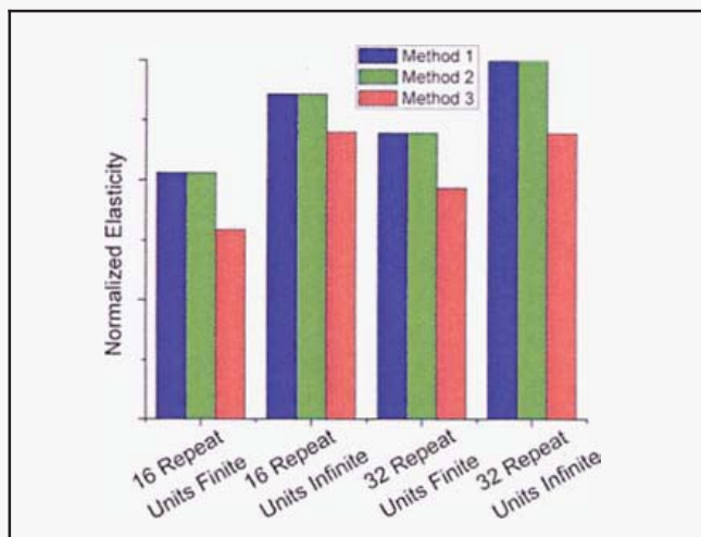
5. Comparison of three methods for calculating axial elasticity in large strain. Data normalized by 122 GPa. Methods 1 (blue) and 2 (green) yield the same result for molecules with different lengths and boundary conditions, while method 3 (red) predicts lower values.
