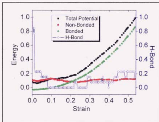
4. A representative plot of potential energy (left y-axis; normalized by 6202 kcal/mol) and corresponding number of hydrogen bonds (right y-axis; normalized by 13) as functions of strain. Data from a simulation of an infinite chain with eight repeat units.
