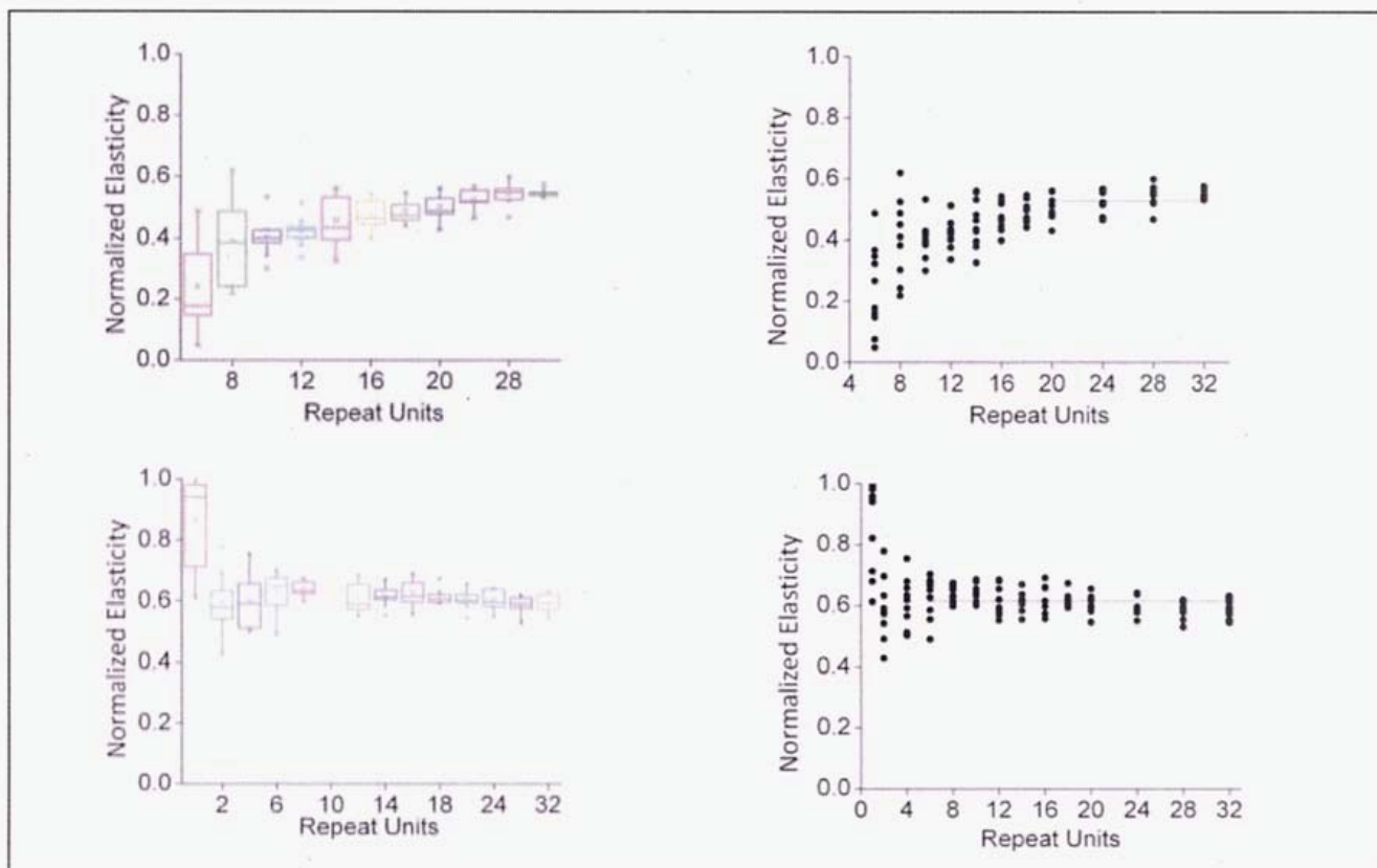
6. Finite (top) and infinite (bottom) molecules at large strain; axial modulus normalized by 177 GPa (the highest value from calculation). The plots on the right show the raw data with a solid line indicating convergence, and left ones provide a statistical representation. Ten independent simulations were run for each case.
