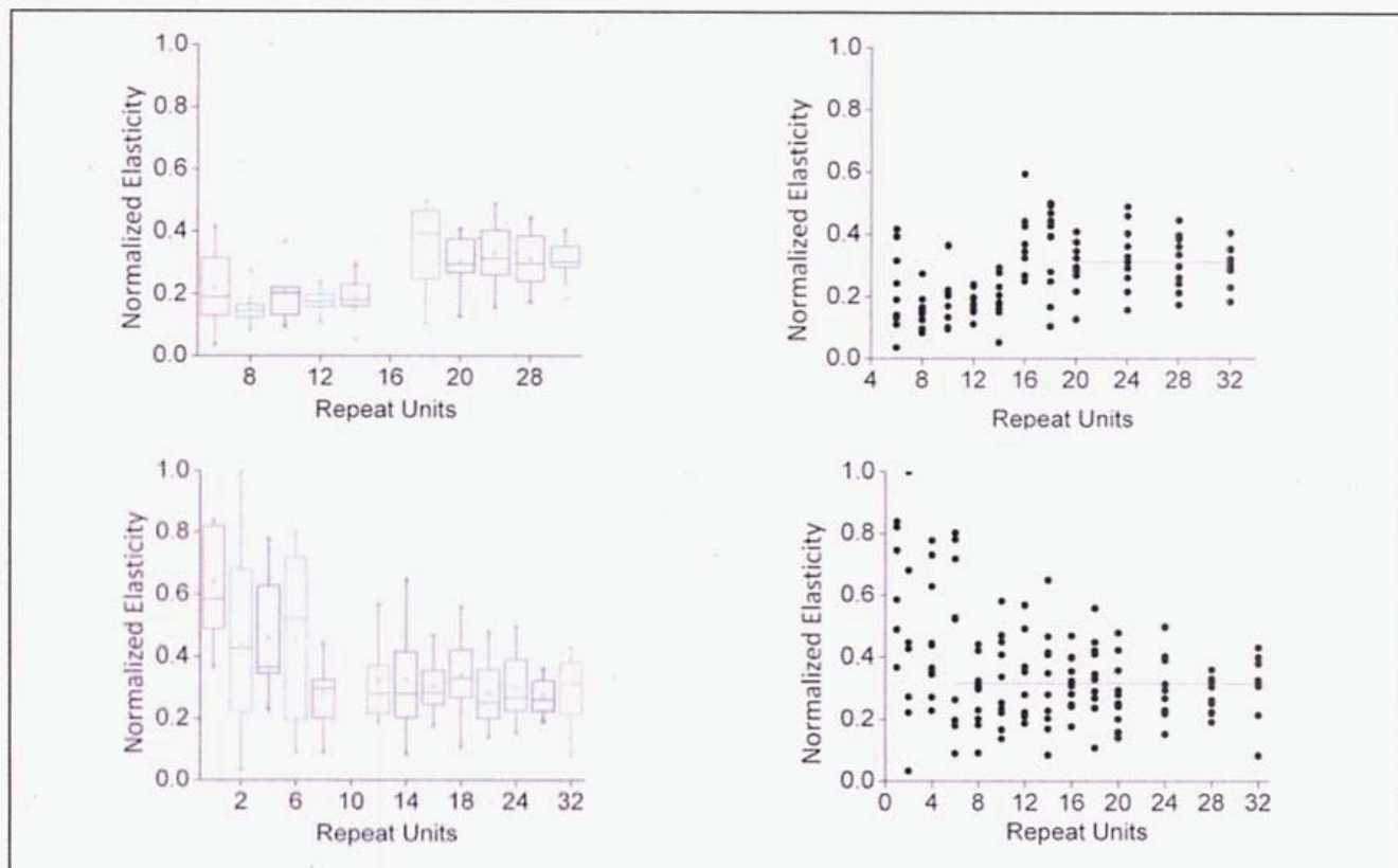
7. Finite (top) and infinite (bottom) molecules at small strain; axial modulus normalized by 802 GPa (the highest value from calculation). The plots on the right show the raw data with a solid line indicating convergence and left ones provide a statistical representation. Ten independent simulations were run for each case.
