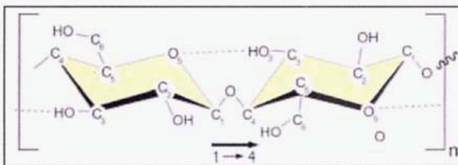
1. Schematic of single cellulose chain repeat unit, showing the directionality of the 1→4 linkage and intramolecule hydrogen bonding (dotted lines).
