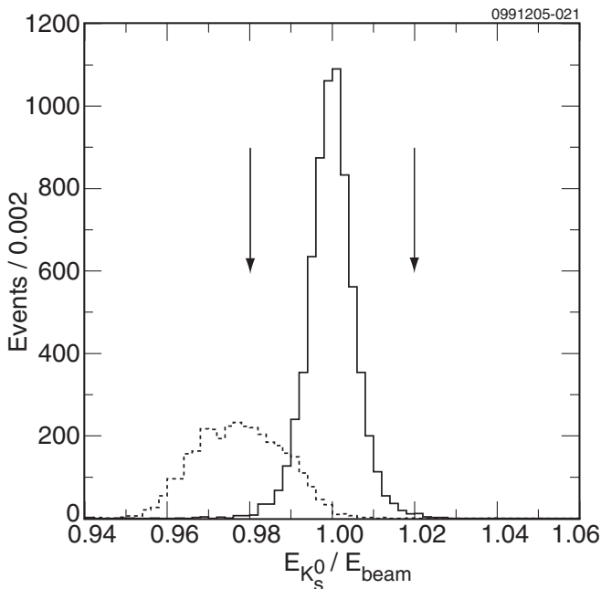
FIG. 1. The scaled K_S^0 energy ( E_{K_S^0}/E_{\text{beam}} ) distribution for the \psi(3770) simulation samples corresponding to the signal (solid histogram) and radiative return (dotted histogram) processes using arbitrary normalization. The arrows mark the signal region.
