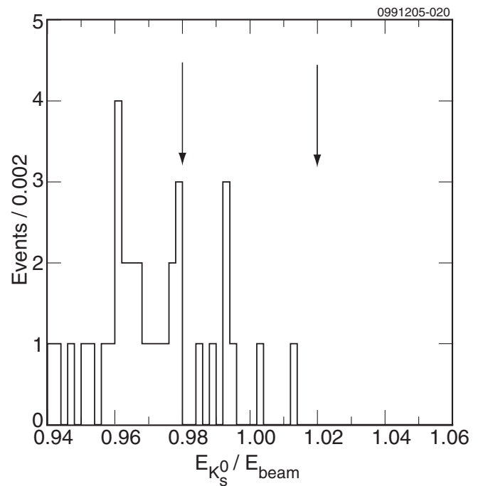
FIG. 2. The scaled K_S^0 energy ( E_{K_S^0}/E_{\text{beam}} ) distribution for the \psi(3770) \rightarrow K_S^0 K_L^0 decay in 281 \text{ pb}^{-1} of data. The arrows mark the signal region.
