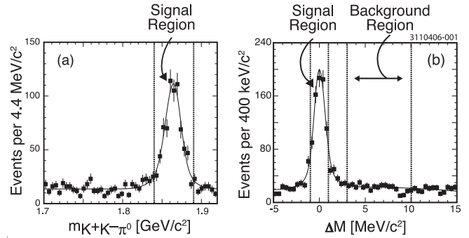
FIG. 1. Distribution of (a) m_{K^+K^- \pi^0} for |\Delta M| < 1 MeV/c 2 and (b) \Delta M for 1.84 < m_{K^+K^- \pi^0} < 1.89 GeV/c 2 after passing all other selection criteria discussed in the text. The solid curves show the results of fits to the m_{K^+K^- \pi^0} and \Delta M distributions, respectively. The vertical lines in (a) and the left-most set of vertical lines in (b) denote the signal region. The right-most set of vertical lines in figure (b) denote the \Delta M sideband used for estimation of the background shape.
