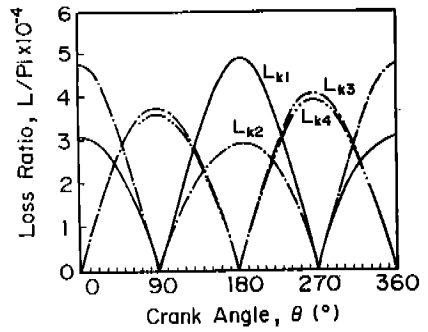
Fig.7 Calculated Key Losses
