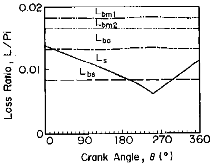
Fig.6 Calculated Losses
