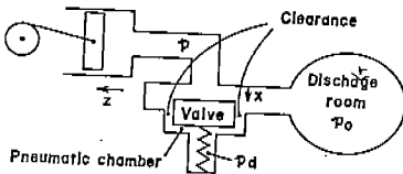
Fig. 1 Discharge valve
