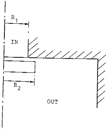
FIGURE 1 DISC VALVE SYMMETRICAL HALF
