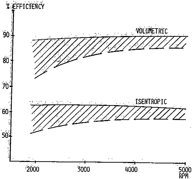
FIG. 9: PERFORMANCE OF TWIN-SCREW COMPRESSOR DISPLACEMENT = 22.3 M 3 /H (13.1 CFM) AT 3000 RPM R 12, COND. TEMP. = 32°C (89.6°F) EVAP. TEMP. = -23.5°C (-10.3°F) PRESSURE RATIO = 6 V_1 = 3.5
