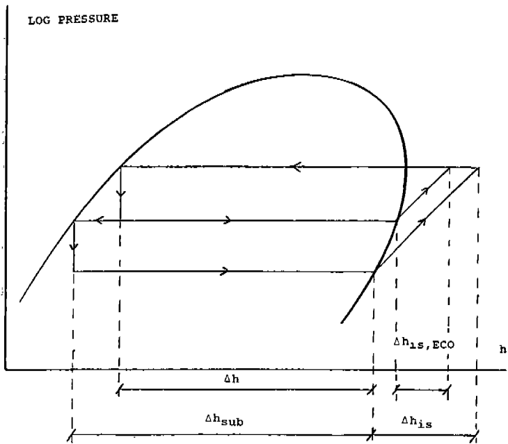
FIG. 5: DEFINITIONS OF ENTHALPIES
