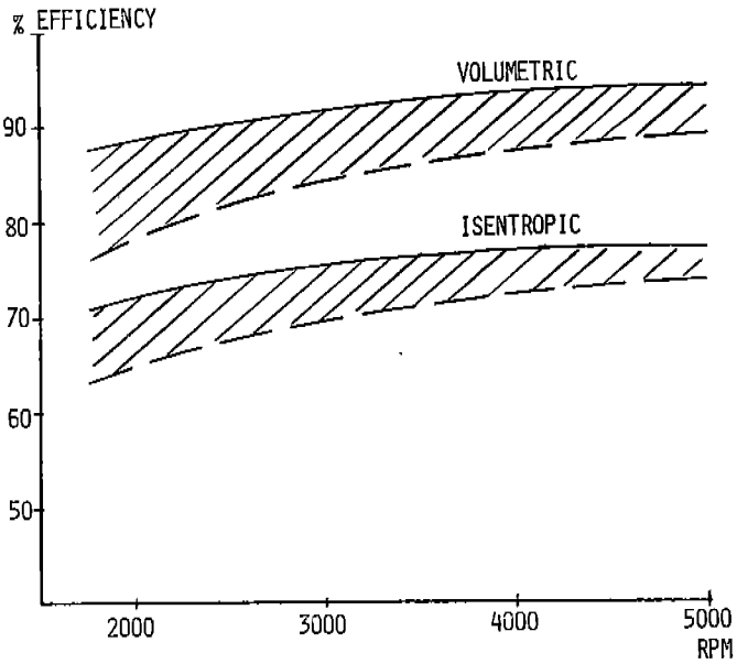
FIG. 8: PERFORMANCE OF TWIN-SCREW COMPRESSOR DISPLACEMENT = 22.3 \text{ m}^3/\text{h} (13.1 CFM) AT 3000 RPM R 22, COND. TEMP. = 50^\circ\text{C} ( 122^\circ\text{F} ) PRESSURE RATIO = 3.0 V_1 = 2.7
