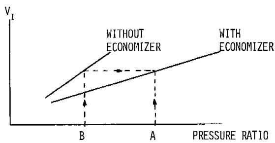
FIG. 4: PRINCIPLE OF V_1 -CORRECTION FOR ECONOMIZER OPERATION
