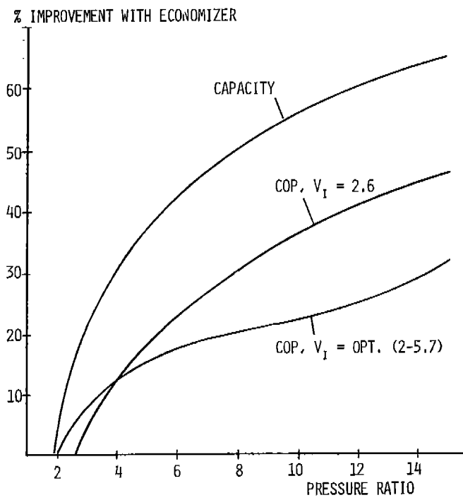
FIG. 3: PERFORMANCE COMPARISON, WITH AND WITHOUT ECONOMIZER R 22, COND. TEMP, = 54.4°C (130°F)
