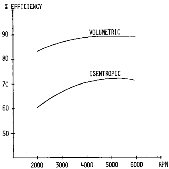
FIG. 10: PERFORMANCE FOR SMALL BOOSTER COMPRESSOR DISPLACEMENT = 59.5 \text{ m}^3/\text{H} (35 CFM) AT 3000 RPM R 22, COND. TEMP. = -6.67^\circ\text{C} ( 20^\circ\text{F} ) EVAP. TEMP. = -34.4^\circ\text{C} ( -30^\circ\text{F} ) V_I = 2.5
