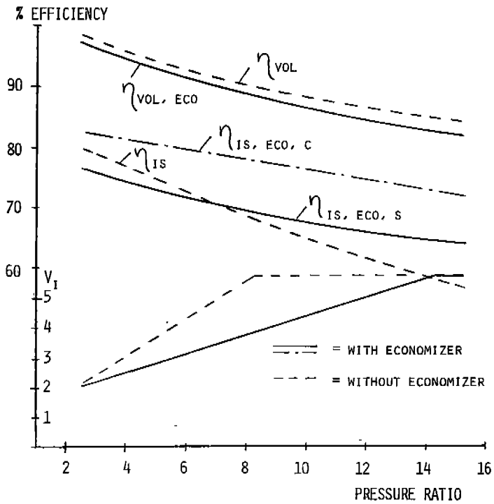
FIG. 7: PERFORMANCE WITH ECONOMIZER DISPLACEMENT = 175,3 m 3 /H (103.2 CFM) AT 3550 RPM R 22, COND. TEMP. = 40,6°C (105°F)
