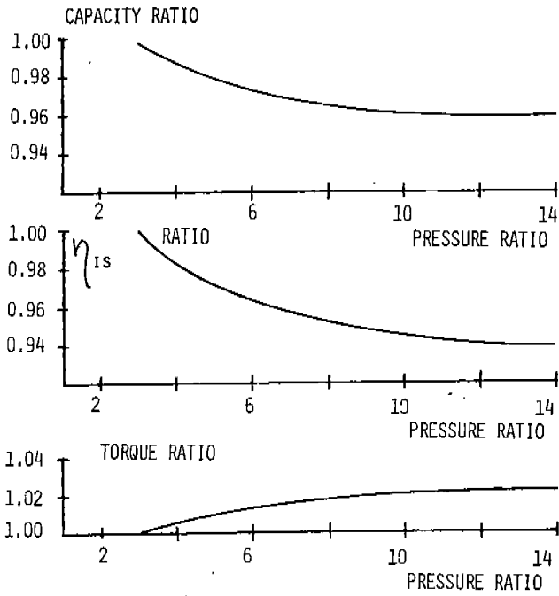
FIG. 1: PERFORMANCE LOSS WITH LIQ. REF. INJECTION R 22, COND. TEMP. = 54.4°C (130°F) V_1 = 2-5.7 INTERNAL COOLING (LIQ. INJ.) COMPARED WITH EXTERNAL COOLING (WATER COOLED OIL)
