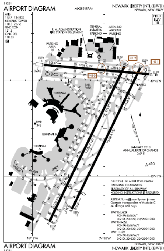
Figure 2.2 Diagram of Newark Liberty International Airport (Federal Aviation Administration, 2014b). Reprinted under public domain.
