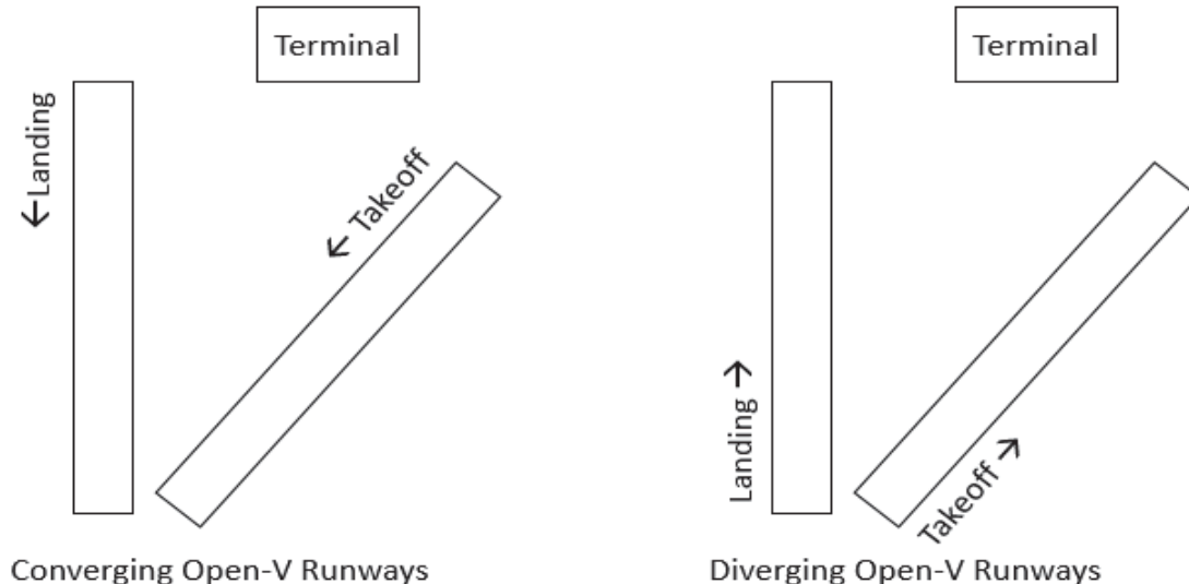
Figure 2.6 Open-V Runway Configurations
