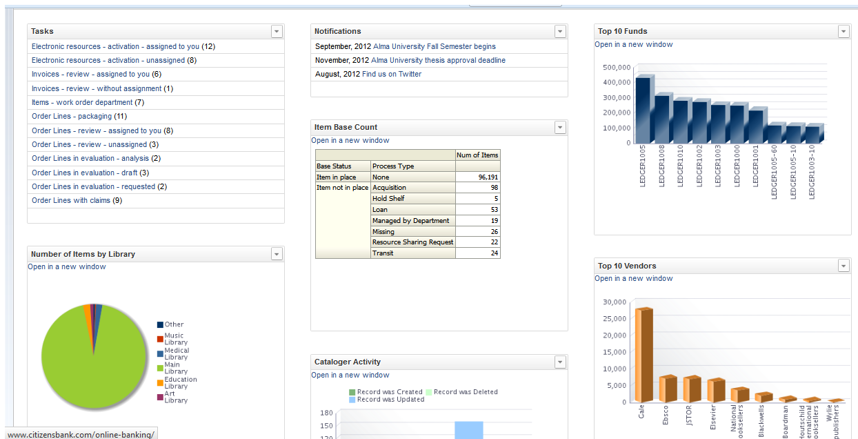
Figure 1. Alma Dashboard
