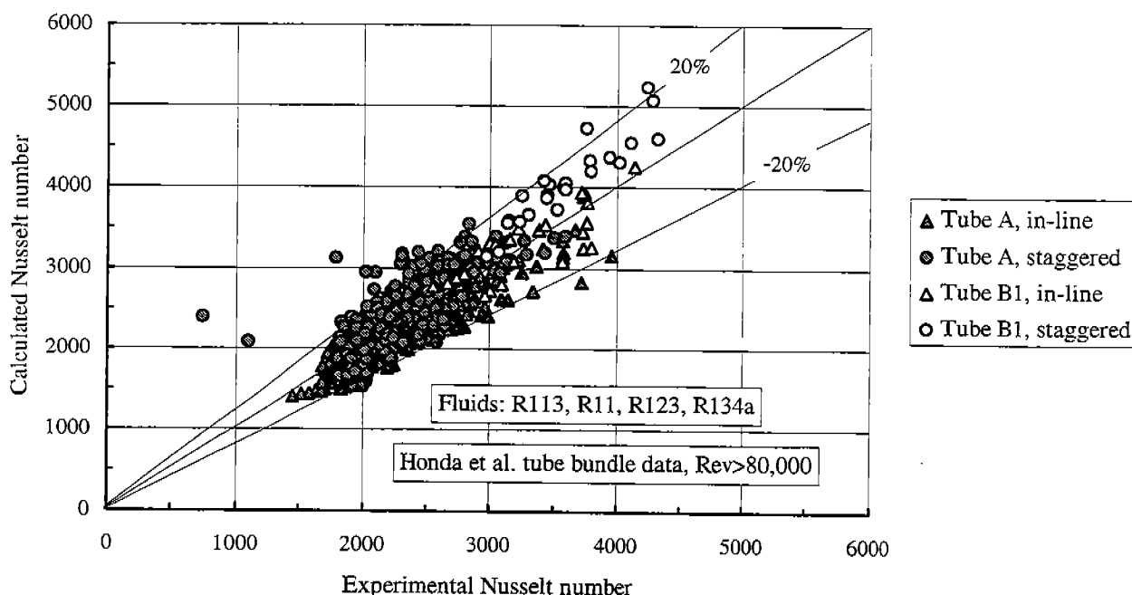
Figure 3. Comparison between the experimental and calculated Nusselt numbers by suggested model (eq. 6).
