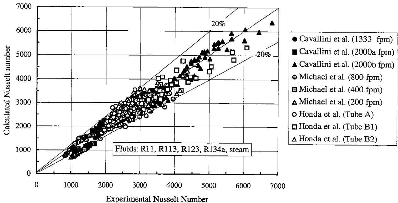
Figure 1. Comparison between the experimental and calculated Nusselt numbers (eq. 1-4).
