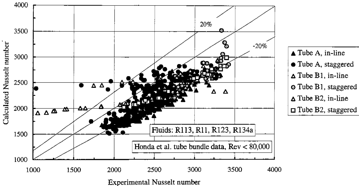
Figure 2. Comparison between the experimental and calculated Nusselt numbers by modified Briggs & Rose model.
