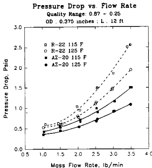
Figure 7. Pressure drop vs. mass flow rate
