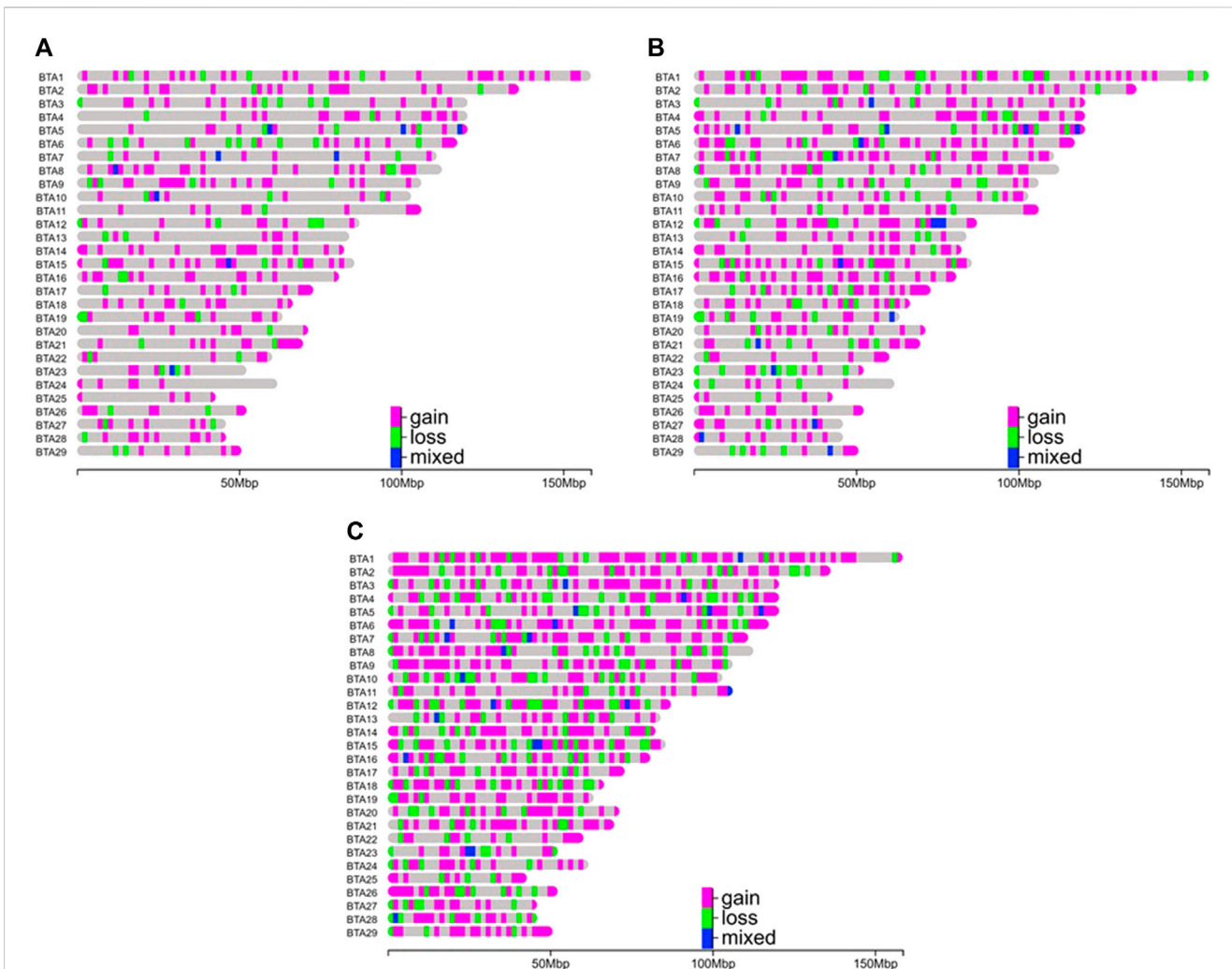
FIGURE 2 Distribution of copy number variation regions (deletions or losses, duplications or gains, and mixed type) by chromosome and selection line. (A) Nellore Control (NeC); (B) Nellore Selection (NeS); (C) Nellore Traditional (NeT).
