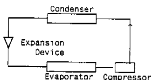
Fig. 1 (a) Block diagram of vapour compression cycle
