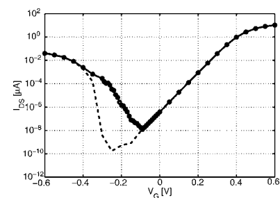
FIG. 4. Current vs gate voltage, for V_d = 0.1 : Without scattering (dashed line); with phonon scattering (solid line with circles). The doping density is 6 \times 10^8 /m.
