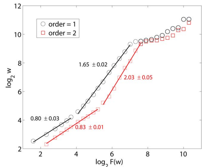
Figure 5. Adaptive fractal analysis of sunspot numbers with polynomial order 1 and 2. doi:10.1371/journal.pone.0024331.g005
