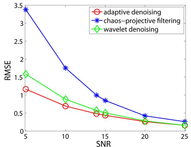
Figure 3. Root Mean Square Error (RMSE) vs. Signal-to-Noise Ratio (SNR) curves for three types of filters (adapted from [7]). doi:10.1371/journal.pone.0024331.g003
