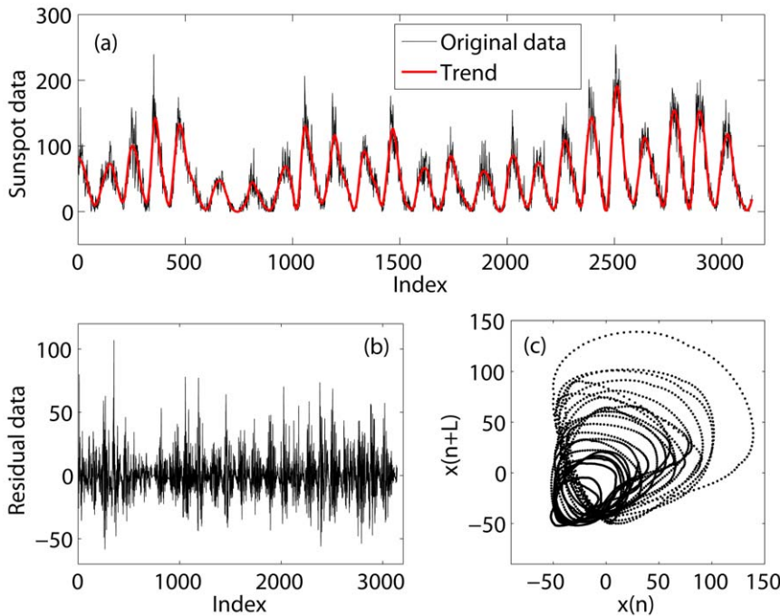
Figure 4. Sunspot data and its trend. (a) original sunspot data (black curve) and the trend data (thick red curve) obtained by adaptive detrending algorithm with a window size of 61 month and a polynomial order of 2; (b) the corresponding residual data; (c) 2-D phase diagram, x(n+L) vs. x(n) with L=30 , for the trend data (with mean removed). doi:10.1371/journal.pone.0024331.g004
