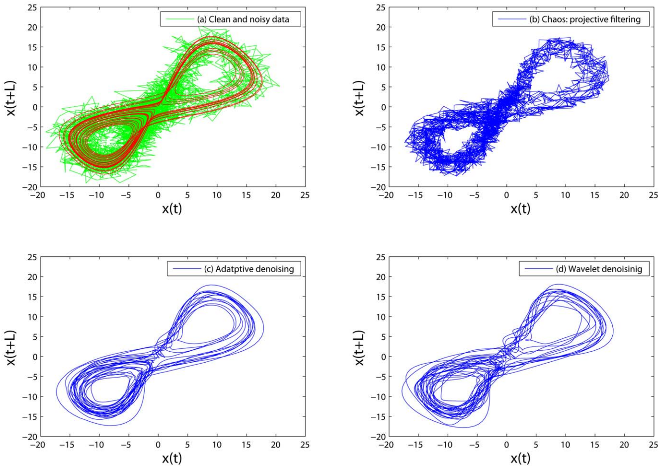
Figure 2. A comparison of proposed adaptive algorithm with wavelet denoising and chaos-based projective filtering for reducing noise in the chaotic Lorenz data. Phase diagrams (i.e., x(t+L) vs. x(t) ) for (a) the clean (red) and noisy (green) Lorenz signal, (b) the signal processed by chaos-based projective filtering, (c) the signal filtered by the proposed adaptive algorithm, and (d) the signal filtered by wavelet denoising. doi:10.1371/journal.pone.0024331.g002
