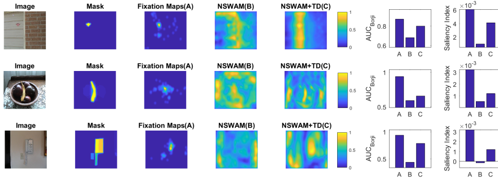
Figure 2: Examples of model output performance given bottom-up only (NSWAM) and with top-down selection (NSWAM+TD). Area Under ROC ( AUC_{Borji} ) compares predictions with human fixations, and the Saliency Index (SI) is calculated as the energy of the a map inside the mask ( S_t ) compared to the one outside the mask ( S_b ), SI=(S_t-S_b)/S_b .
