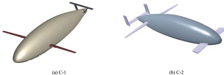
Figure 1. Pictorial views of clean configurations of hybrid buoyant aircraft concepts.
