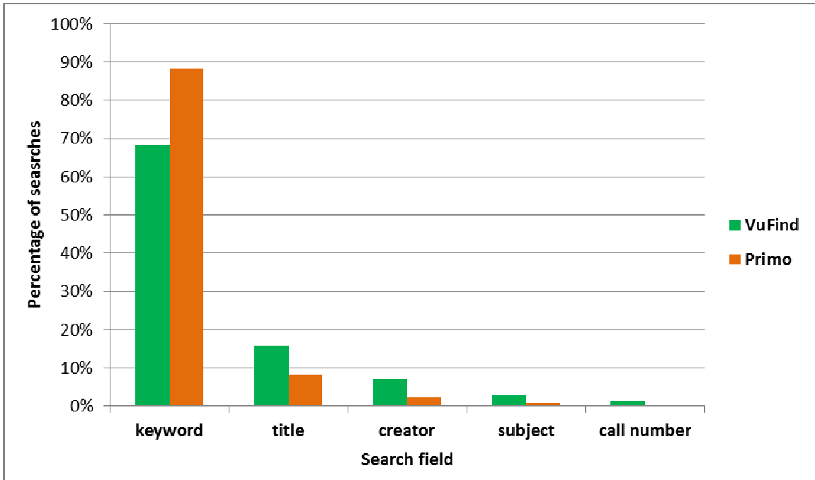
Figure 3. Contrast of common search fields used in VuFind and Primo.
