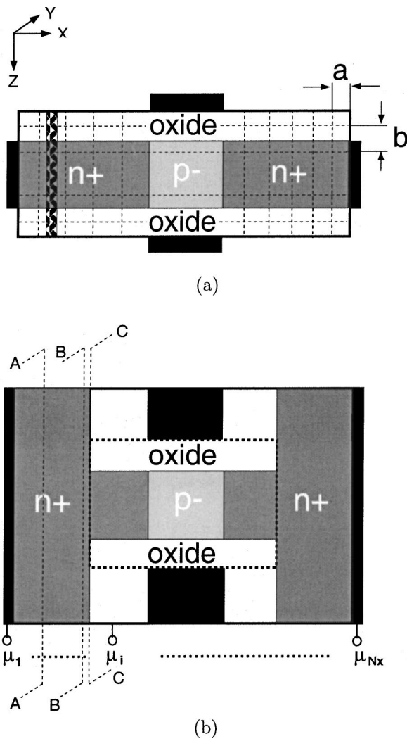
FIG. 1. (a) Ultrathin body DG MOSFET structure with a S/D doping of 10^{20} \text{ cm}^{-3} and an intrinsic channel (channel thickness=1.5 nm). The S/D regions are 20 nm in length, the gate length is 10 nm and the S/D-channel junctions are abrupt. A slice of the device within which a 1D, z directed effective mass equation is solved, is also indicated. (b) A thin body DG MOSFET with abruptly flared out S/D regions. The length of the flared regions is 10 nm, their thickness is 6.2 nm and the overall device length is 50 nm (same as that for device (a)). The region within the dashed box is the intrinsic device.
