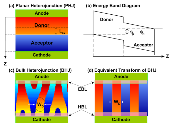
FIG. 1. (Color online) Structure of an organic solar cell. (a) PHJ based OPV cell. (b) The band diagram for PHJ cell at open circuit condition. (c) BHJ type OPV cell. The active layer morphology is generated by numerical simulation. W_D is the average domain size in the structure. (d) Equivalent geometrical transform of the complicated BHJ morphology. The width of the transformed rectangle is same as W_D of BHJ morphology. EBL and HBL are electron and hole blocking layers respectively.
