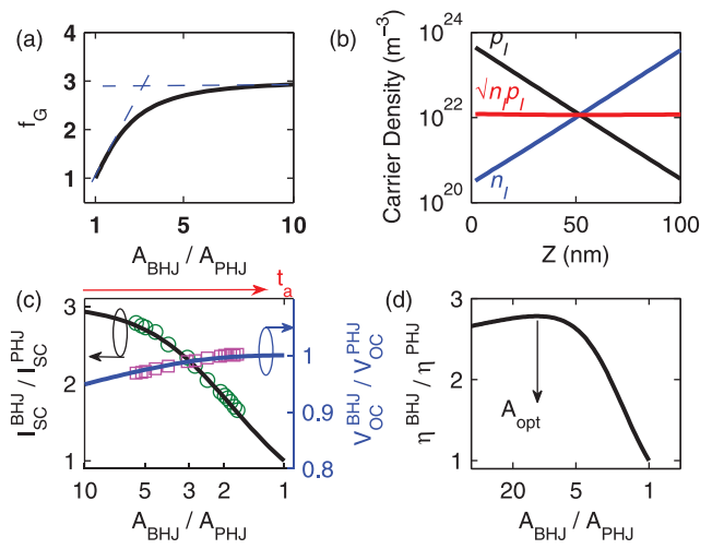
FIG. 2. (Color online) Validation of analytical model (solid line) with detailed numerical simulation (symbols). (a) The geometric amplification function f_G(A_{BHJ}) is plotted. Note that for A_{BHJ} \gg A_{PHJ} , the function f_G saturates to a fixed value given by \eta_D T_{film} / L_{ex} . (b) Interfacial carrier densities as a function of distance from anode to cathode are plotted. We note that product of the interfacial carrier densities remains essentially constant throughout the active volume. (c) Short circuit current ( I_{SC}^{BHJ} ) of BHJ cell normalized by short circuit current ( I_{SC}^{PHJ} ) of PHJ cell is plotted against total D-A interfacial area ( A_{BHJ} ), divided by PHJ cell area ( A_{PHJ} ). Open circuit voltage of BHJ cell ( V_{OC}^{BHJ} ) is also plotted against area of interface on the right hand side axis. (d) The \eta_{BHJ} / \eta_{PHJ} is plotted assuming same FF for both PHJ and BHJ cell.
