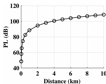
Figure 4. The path loss with change in distance.
