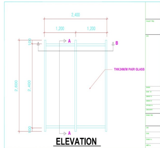
Figure 1. Size of the specimen of glass curtain wall
