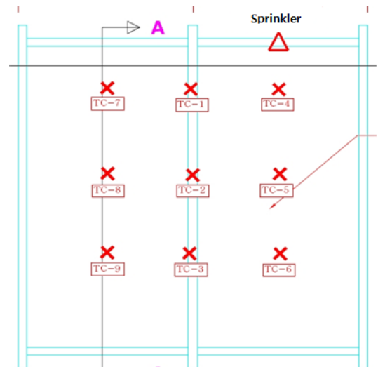
Figure 2. Installation location of temperature surveying line
