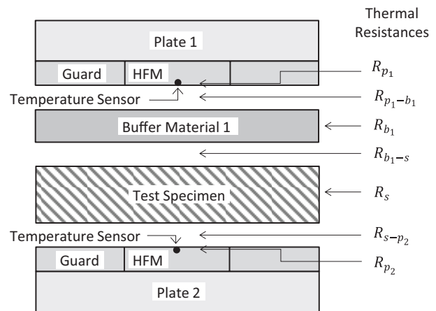
Figure 1. Heat flow meter (HFM) apparatus with specimen and a buffer material present.
